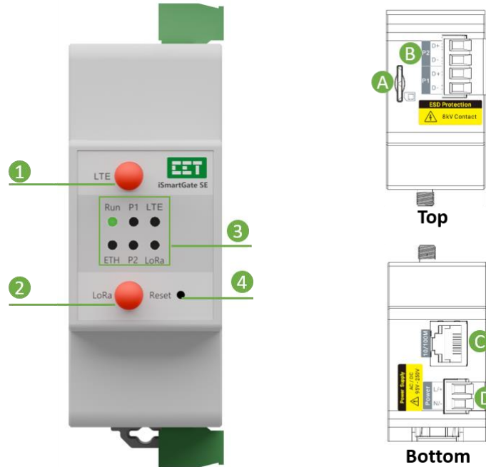
Figure 2-1 Appearance
